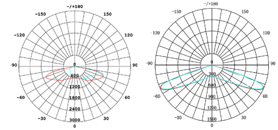
T4M5703 IESNA Type IV Medium
