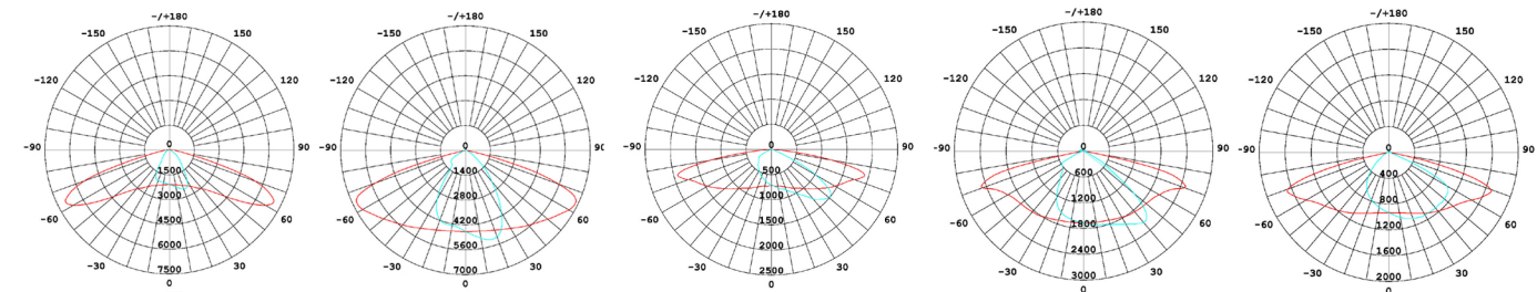
T1S3501 IESNA Type I Short
