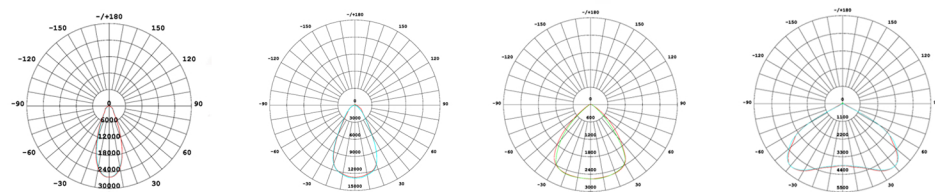
40D3540 Beam Angle(50%)40DEG 60D3560 Beam Angle(50%)60DEG 90D3590 Beam Angle(50%)90DEG 00D1010 Beam Angle(50%)110DEG
