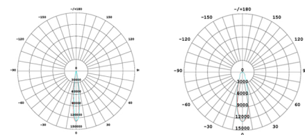
12D1908 Beam Angle(50%)12DEG 25D3725 Beam Angle(50%)25DEG
