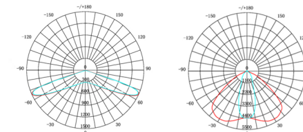
T5S3040 IESNA Type VS Short 11D3030 Beam Angle(50%)110x40DEG
